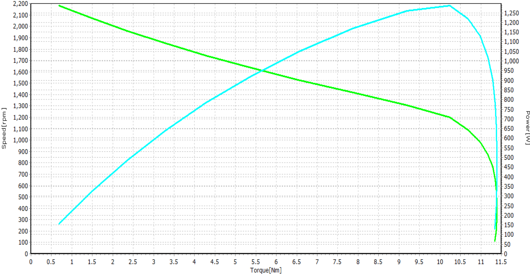
Speed,Power v. Torque
